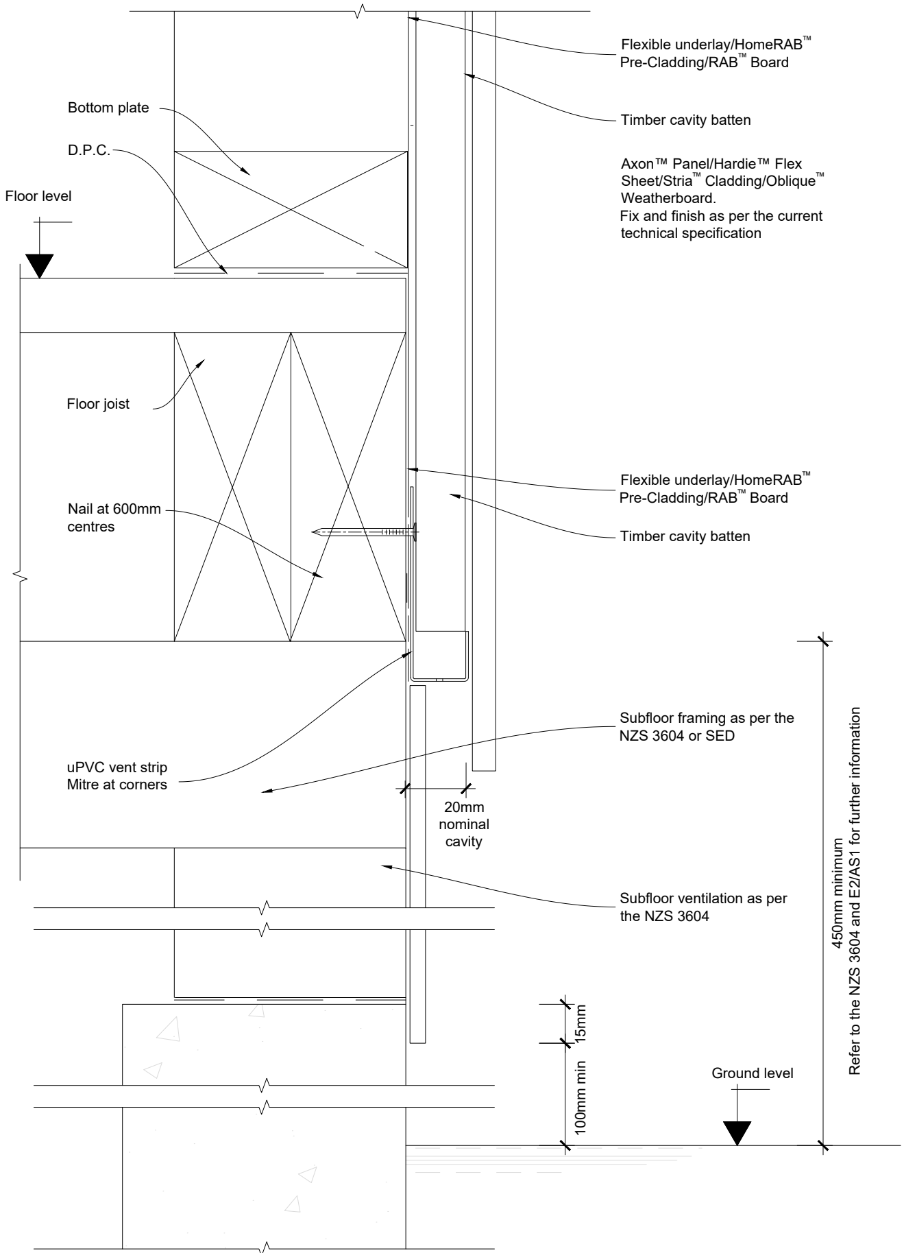
fig41 jhl_junc_c_strc_foun-timb.dwg
